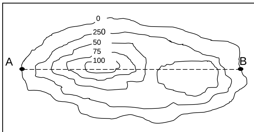
Fig. 5.9: An Island
