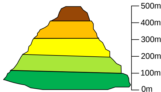
Fig. 5.2: Contour Layering
